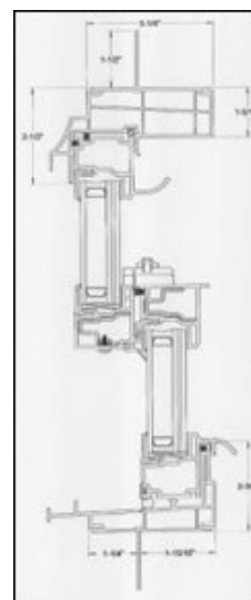
Cross Section
